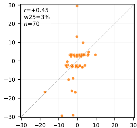
Haiku 4.5
