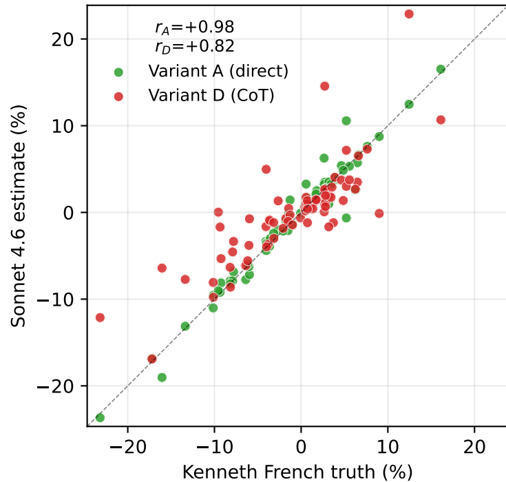
A vs D on matched Mkt-RF months ( n=74 )
