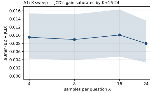
Figure 5. K -sweep on Anthropic Claude-Haiku-4.5 NegChecker forecasts. Non-vanishing \Delta Brier asymptote: the empirical signature of structural incoherence in p_F .
