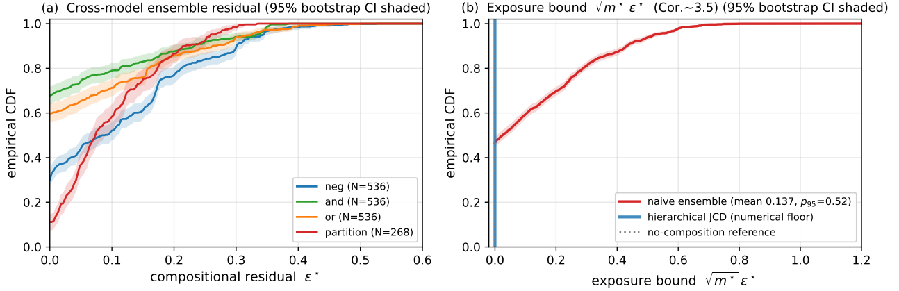
Figure 2. Compositional residuals and the exposure bound. (a) ECDF of \varepsilon^* across N=1,876 ensemble cliques, stratified by relation. Each component is per-call JCD-projected, so any positive \varepsilon^* is cross-component incoherence introduced by composition. (b) ECDF of the exposure bound \sqrt{m^*} \varepsilon^* (Cor. 3.5) under three regimes: naive composition (mean 0.137), hierarchical JCD (at the OSQP floor), and a single-LLM no-composition reference. Shaded bands are 95% bootstrap CIs ( B=1000 ).
