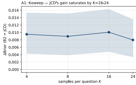
Figure 5. K -sweep on Anthropic Claude-Haiku-4.5 NegChecker forecasts. Non-vanishing \Delta\text{Brier} asymptote: the empirical signature of structural incoherence in p_F .
