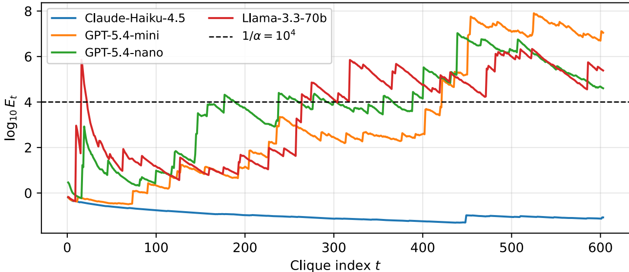
Bounded-difference e-process per model (rejection threshold 1/\alpha = 10^4 )
