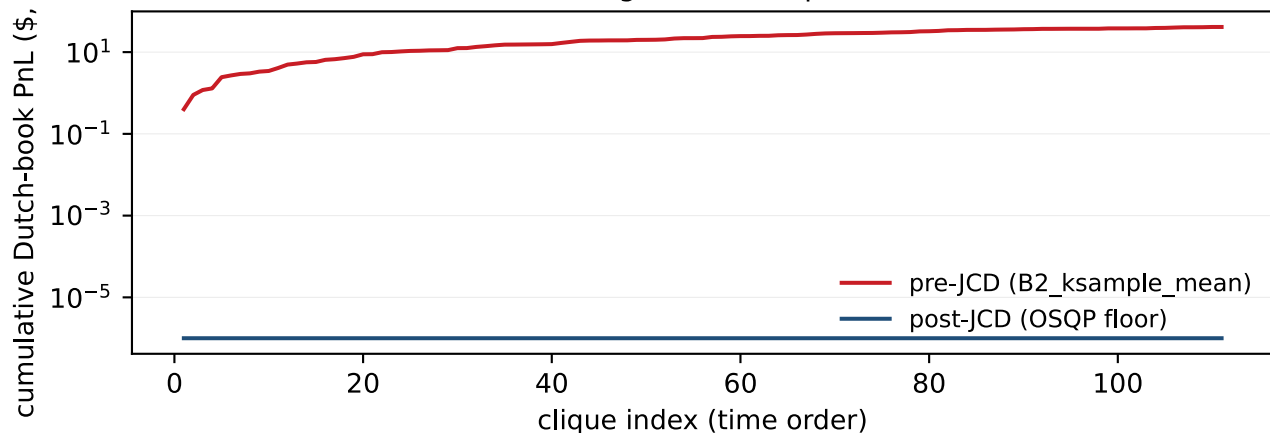
Cumulative Hanson-LMSR arbitrage PnL: collapses to the OSQP numerical floor
