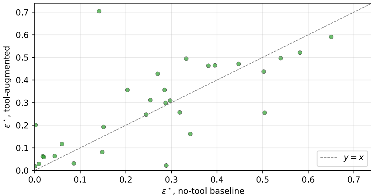
Compositional residual: tool-augmented vs no-tool (N=30 partitions; mean eps* 0.260 -> 0.283)
