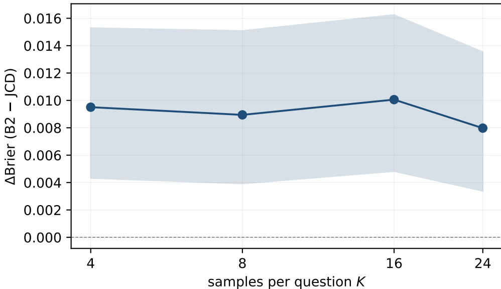
A1: K-sweep — JCD's gain saturates by K \approx 16-24
