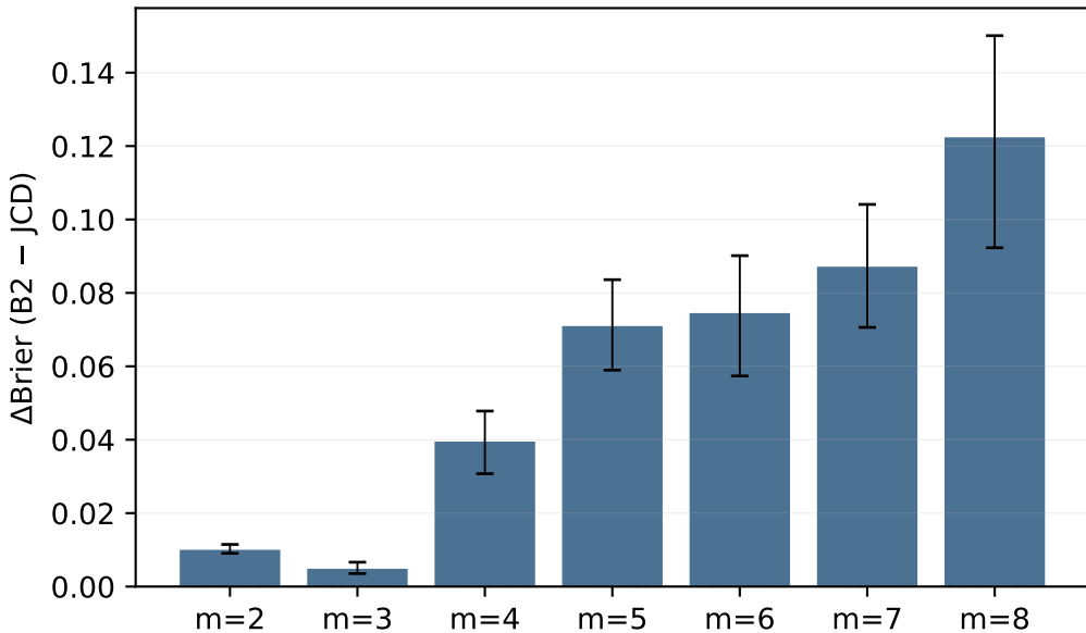
A2: per-clique-size breakdown
