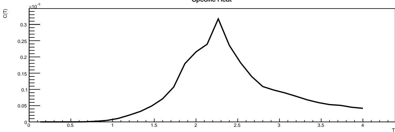
Specific Heat
