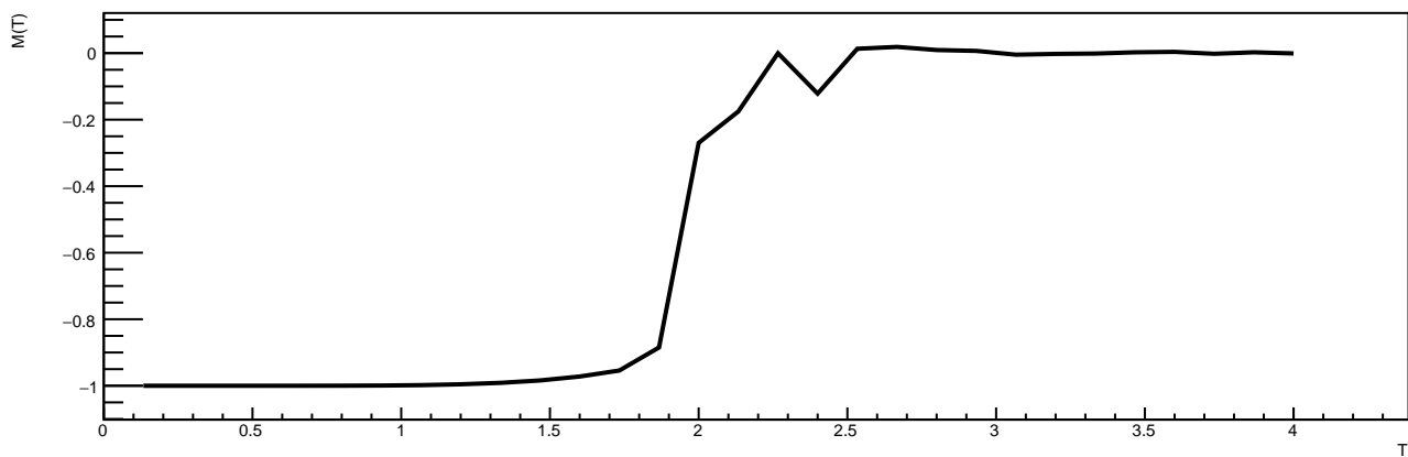
Magnetization
