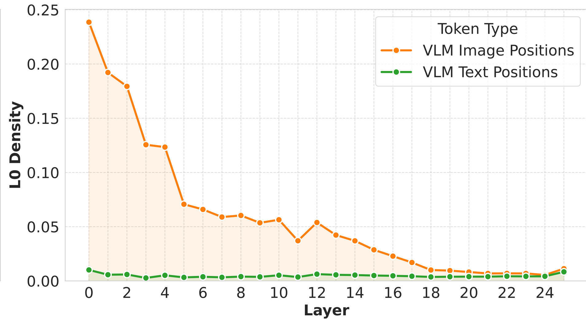
SAE Active Feature Fraction Across Layers
