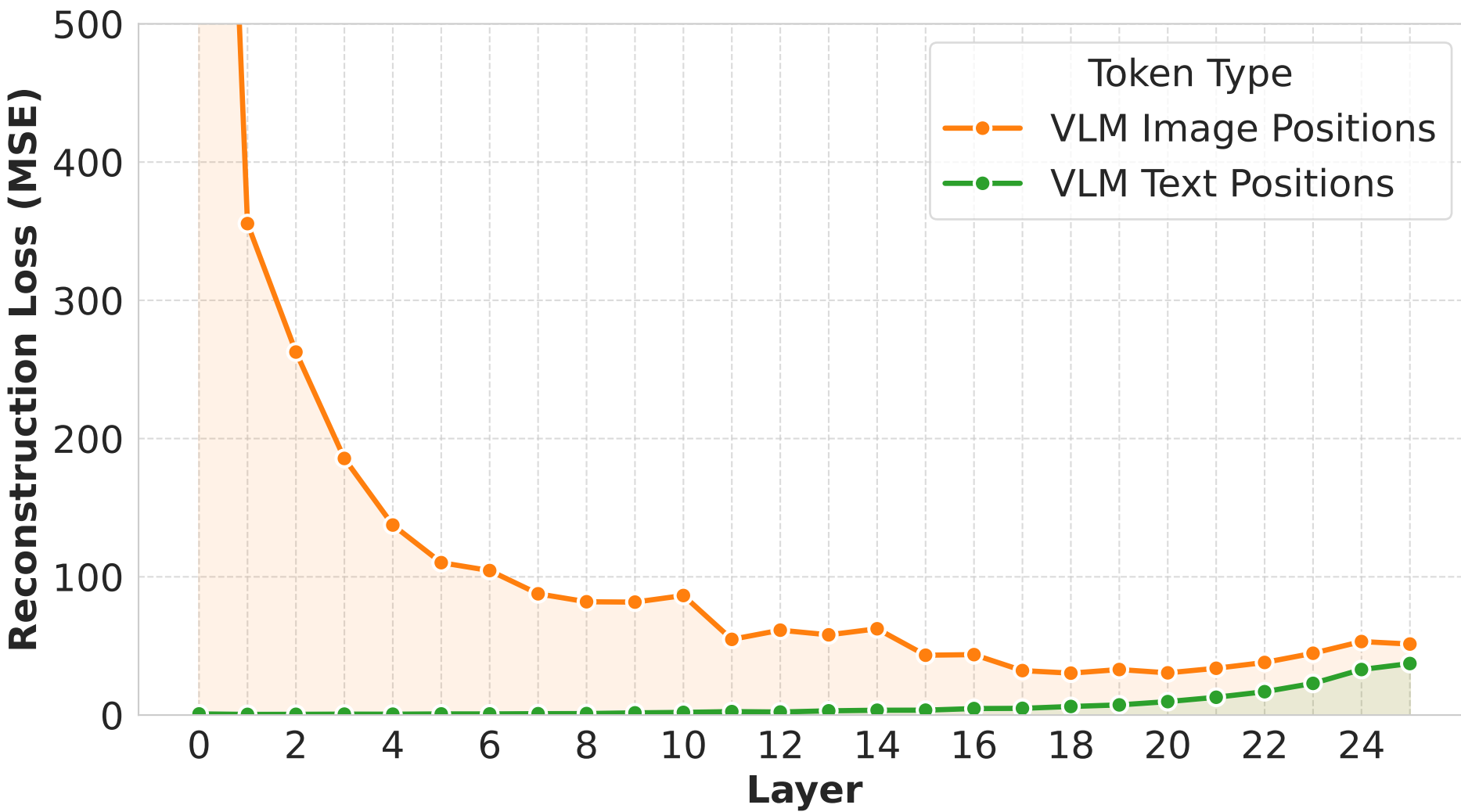
SAE Reconstruction Loss Across Layers
