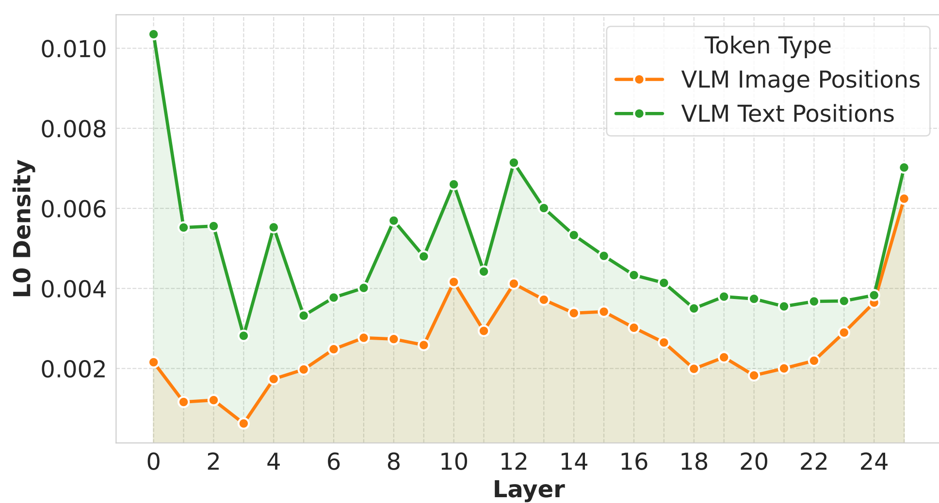
SAE Active Feature Fraction Across Layers
