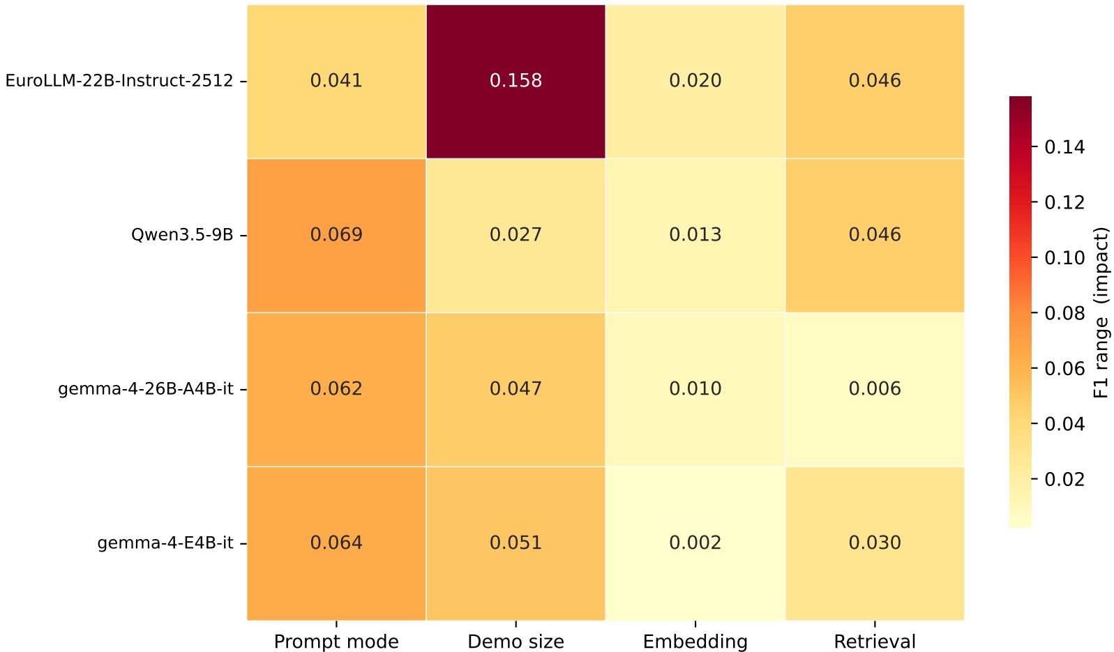
Impact of each configuration axis on F1 Macro (range of per-value marginal means, per model)
