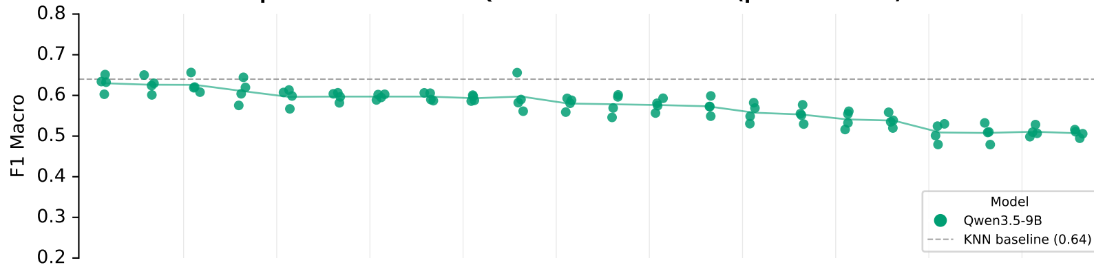
Specification Curve — Qwen3.5-9B — F1 Macro (points + mean)
