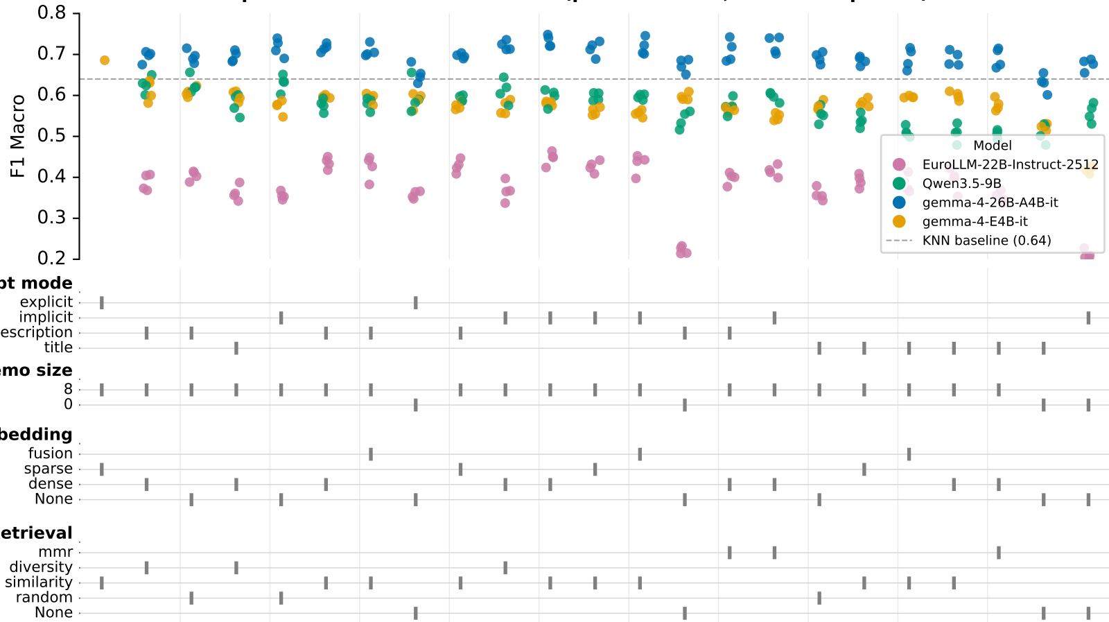
Specification Curve — F1 Macro (points + mean, all models pooled)
