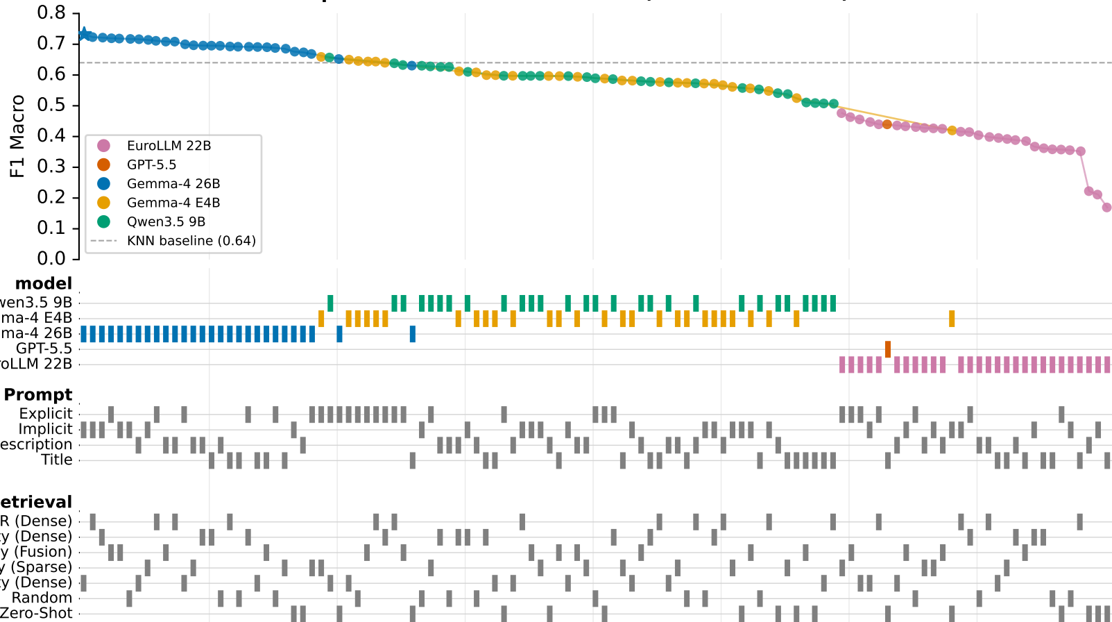
Specification Curve — F1 Macro (mean across folds)
