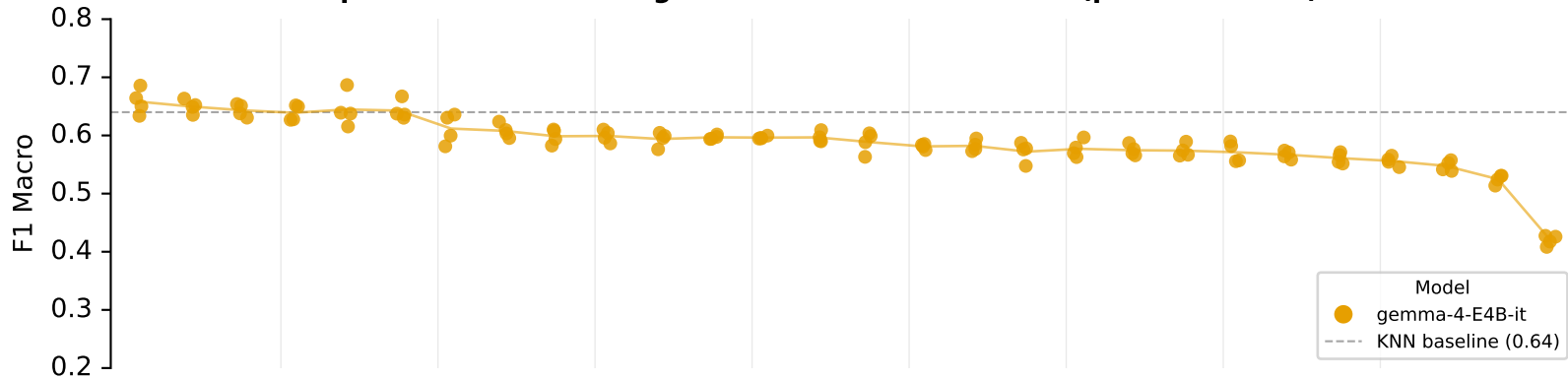
Specification Curve — gemma-4-E4B-it — F1 Macro (points + mean)
