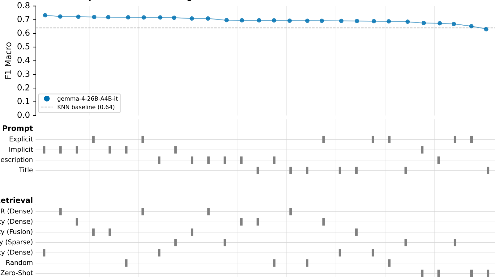
Specification Curve — gemma-4-26B-A4B-it — F1 Macro (mean across folds)
