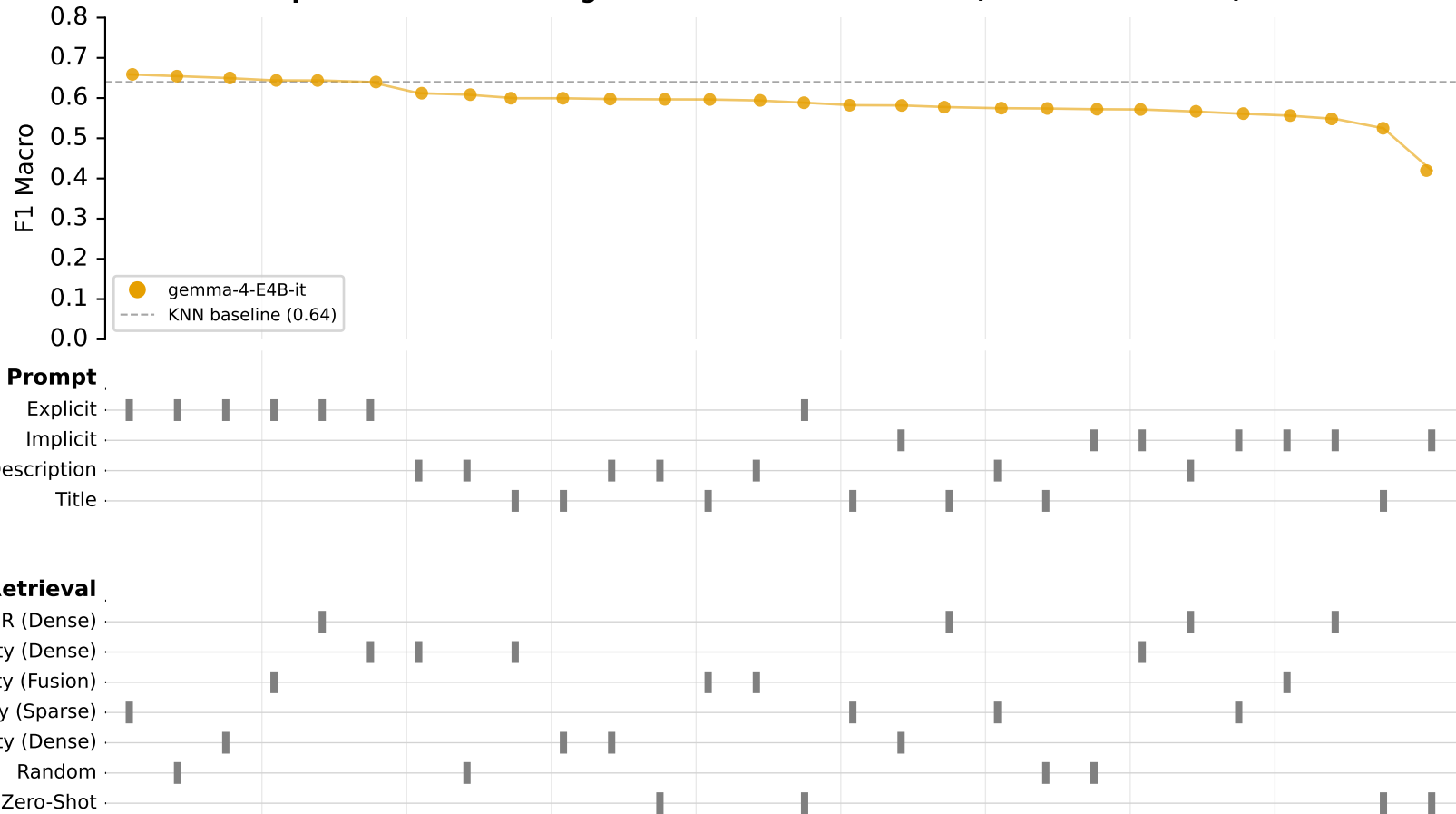
Specification Curve — gemma-4-E4B-it — F1 Macro (mean across folds)
