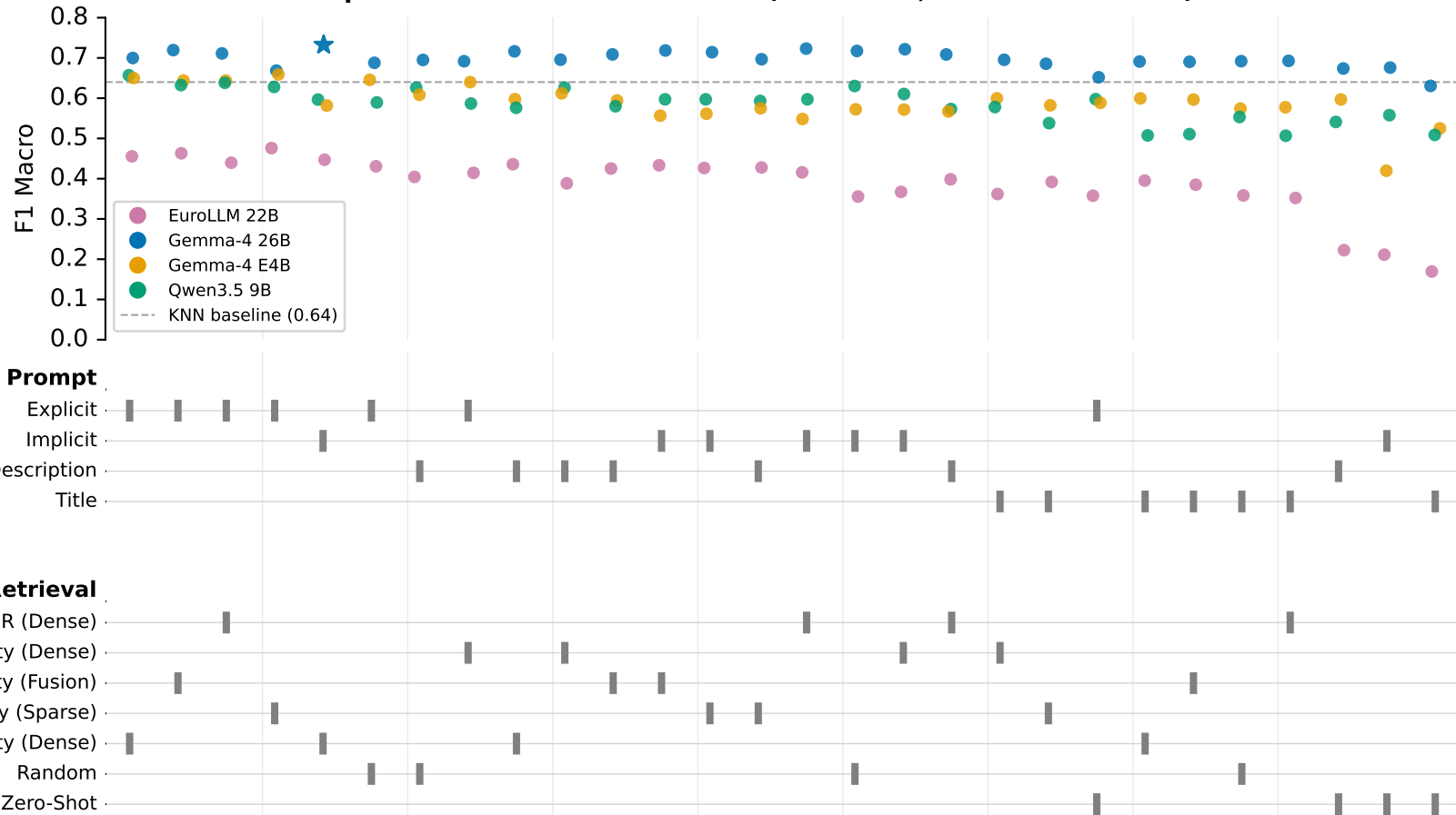
Specification Curve — F1 Macro (all models, mean across folds)
