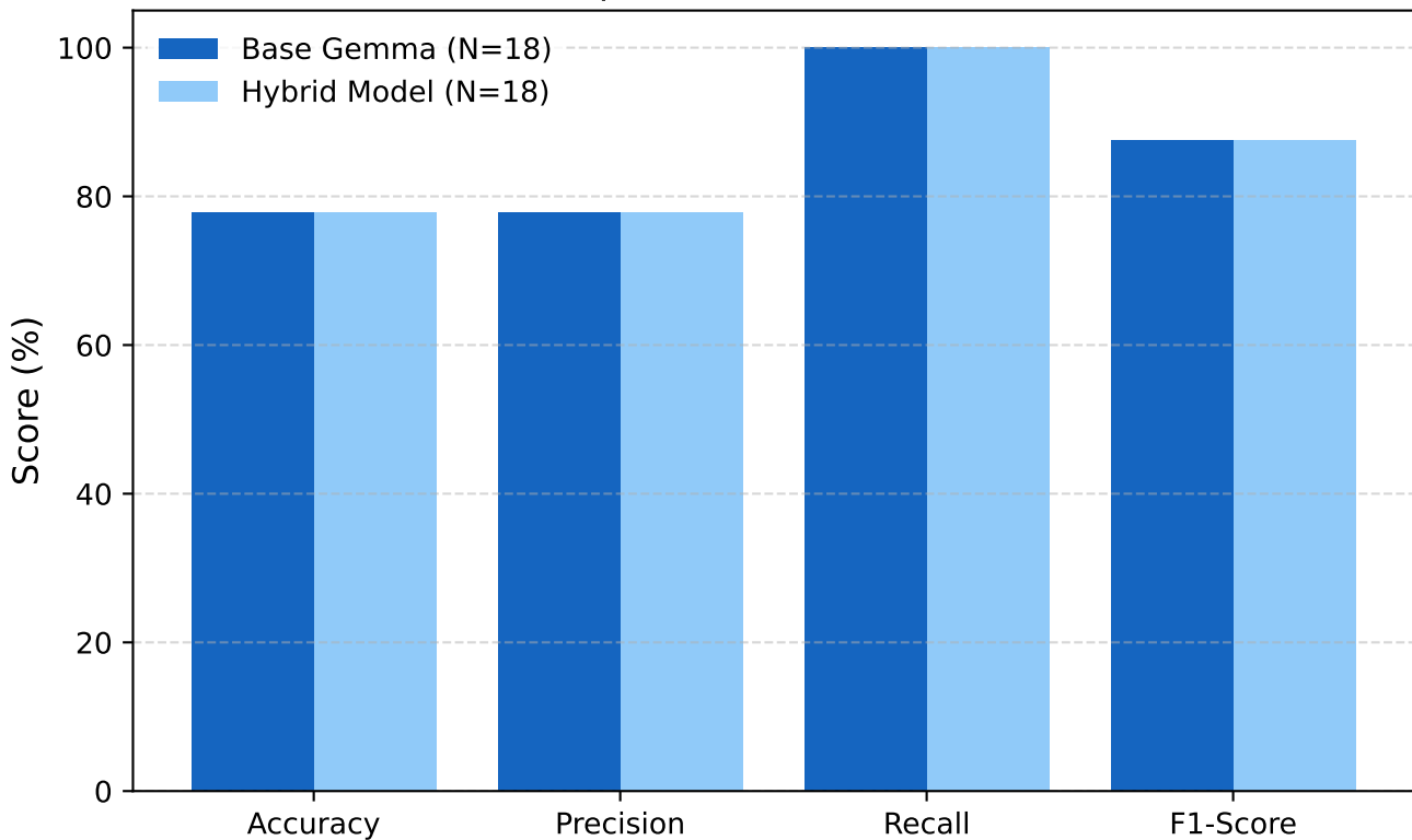
Head-to-Head Comparison on Common Executed Subset
