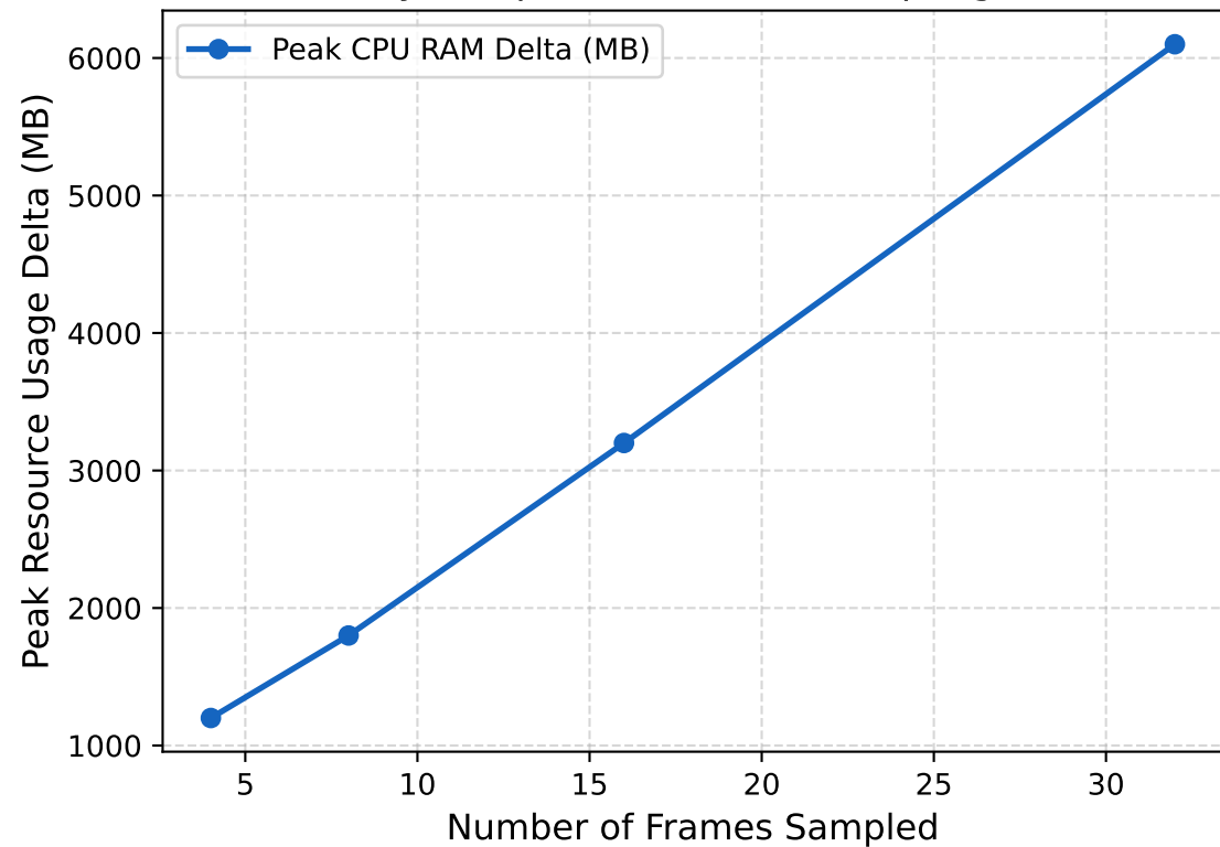
Memory Footprint vs. Frame Sampling Count
