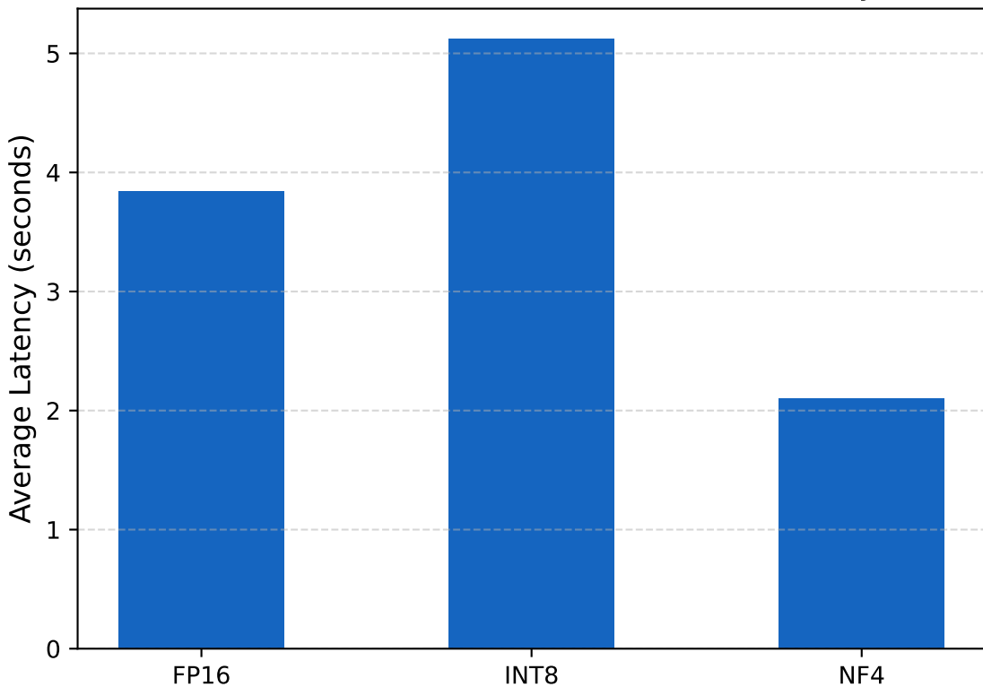
Quantization Precision vs. Inference Latency
