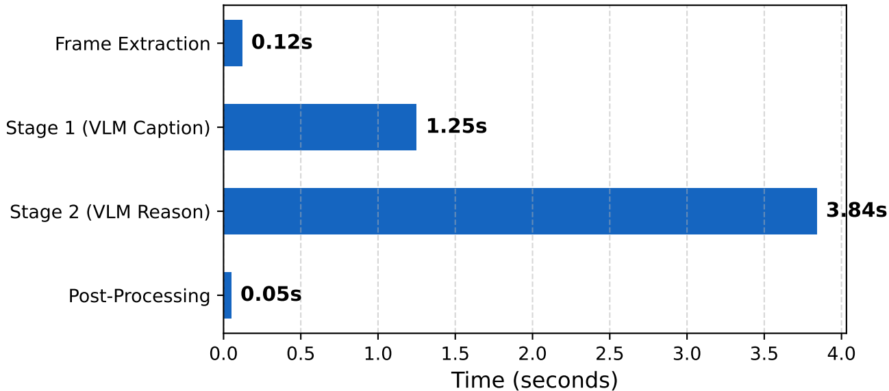
VLM Pipeline Execution Profile Breakdown
