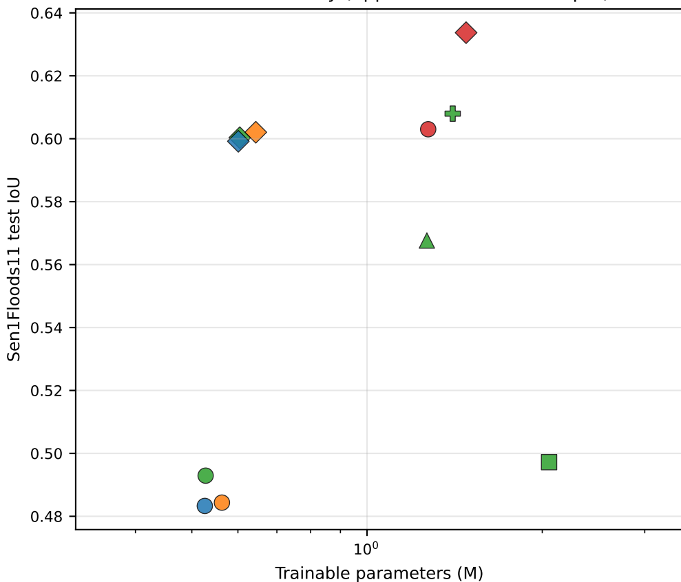
Parameter efficiency (upper-left is the sweet spot)
