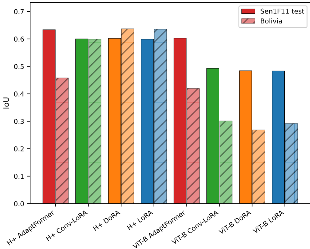
Per-method IoU: in-dist. (solid) vs. Bolivia (hatched)
