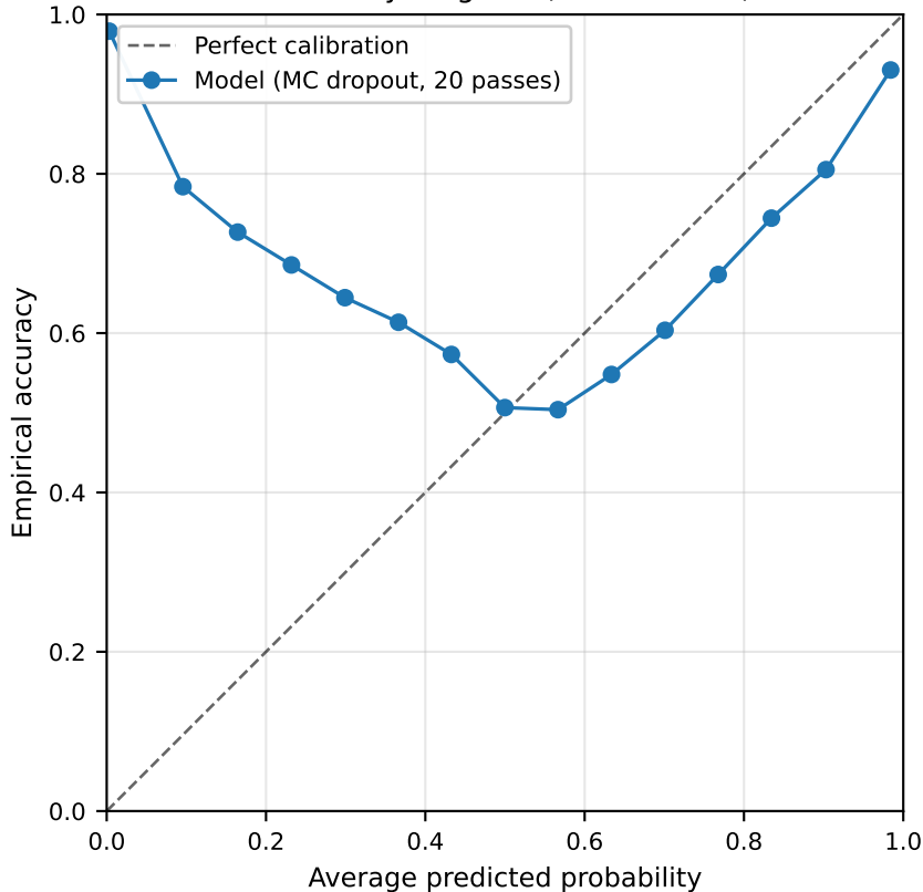
Reliability diagram (ECE = 0.847)
