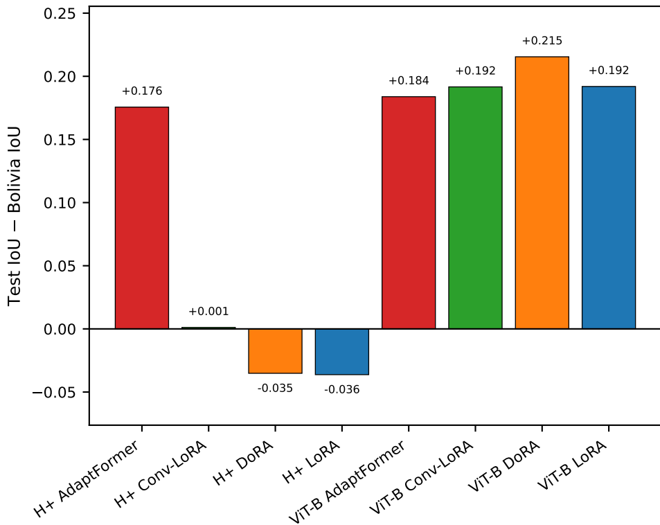
OOD generalization gap (smaller is better)
