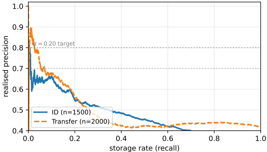
CAEM storage precision vs storage rate
