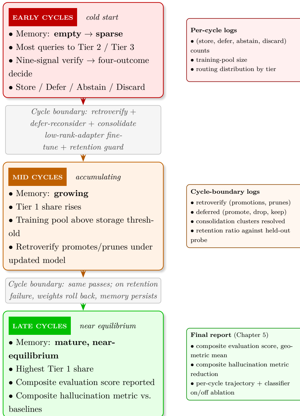
Figure 1.2: Self-improvement trajectory shown schematically as early, mid, and late phases; six cycles realised under the ten-cycle registered cap and closed under the equilibrium-saturation gate at the cycle-five close. Each phase runs the per-query pipeline (Stages 1 to 7, including the Stage 3b retrieval-utility classifier that refines the retrieval-augmented dispatch into either the zero-shot tier or the retrieval-augmented tier on a per-query basis) with nine-signal post-generation verification and the four-outcome storage decision over a fresh workload. At each cycle boundary (Stage 8) a retroactive re-verification pass refreshes stored composites under the updated generator, a deferred-entry reconsideration pass sweeps the deferred buffer, a memory consolidation pass collapses near-duplicate episodes, low-rank-adaptation fine-tuning draws from a strict training pool through a benchmark-balancing reweighting layer, and a multi-modal retention probe panel spanning a general-knowledge multiple-choice surface, an open-text factoid surface, and a commonsense multiple-choice surface aborts the cycle with an adapter rollback when the worst probe ratio falls below a fixed floor. Numeric values of the retention floor, the training threshold, the storage cut-point, and related thresholds are specified in Chapter 4. The memory is never rolled back, so accumulated knowledge survives short events. Headline results across
