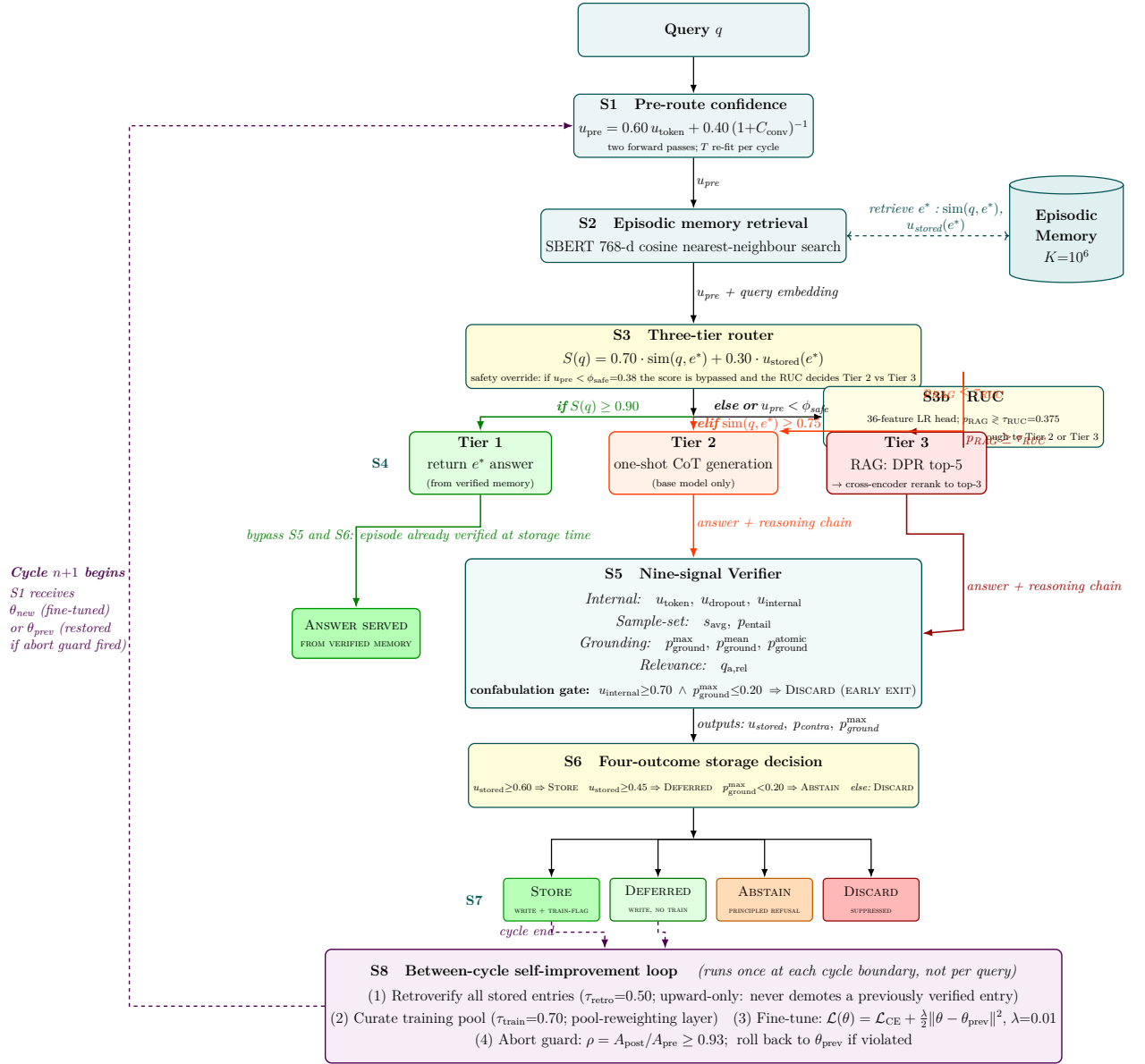
Figure 4.1: The eight-stage CAEM pipeline. Stages S1–S8 are described in Chapter 4; the retrieval-utility classifier (Stage S3b, RUC) of Section 4.2.5 sits between the three-tier router and the retrieval-augmented tier, intercepting the safety-veto and score-formula fall-through dispatches and redirecting retrieval-hurt queries to the zero-shot tier. The nine deployed signals at S5 are the registered set minus h_{\text{norm}} (registered then retired at the cycle-zero audit; see the list-of-symbols footnote) and p_{\text{contra}} (structurally zero under the deployed MiniCheck judge). The outer dashed arrow indicates the cycle-boundary handoff from the close of one cycle to the start of the next.
