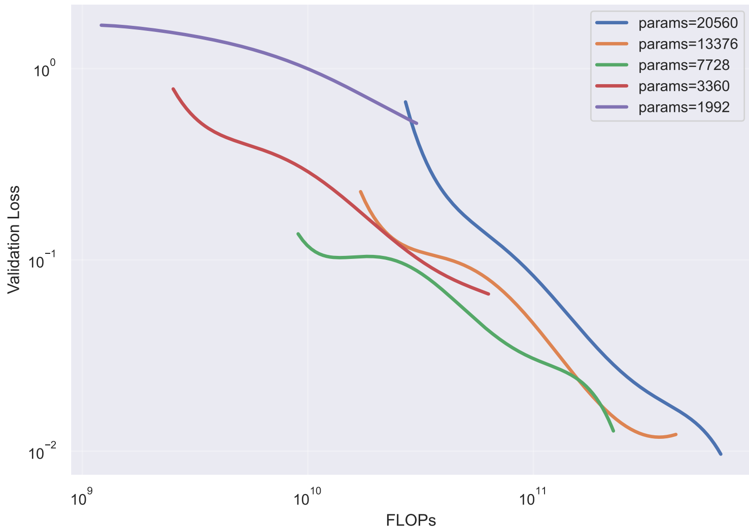
Scaling Law: Validation Loss vs Compute (FLOPs)
