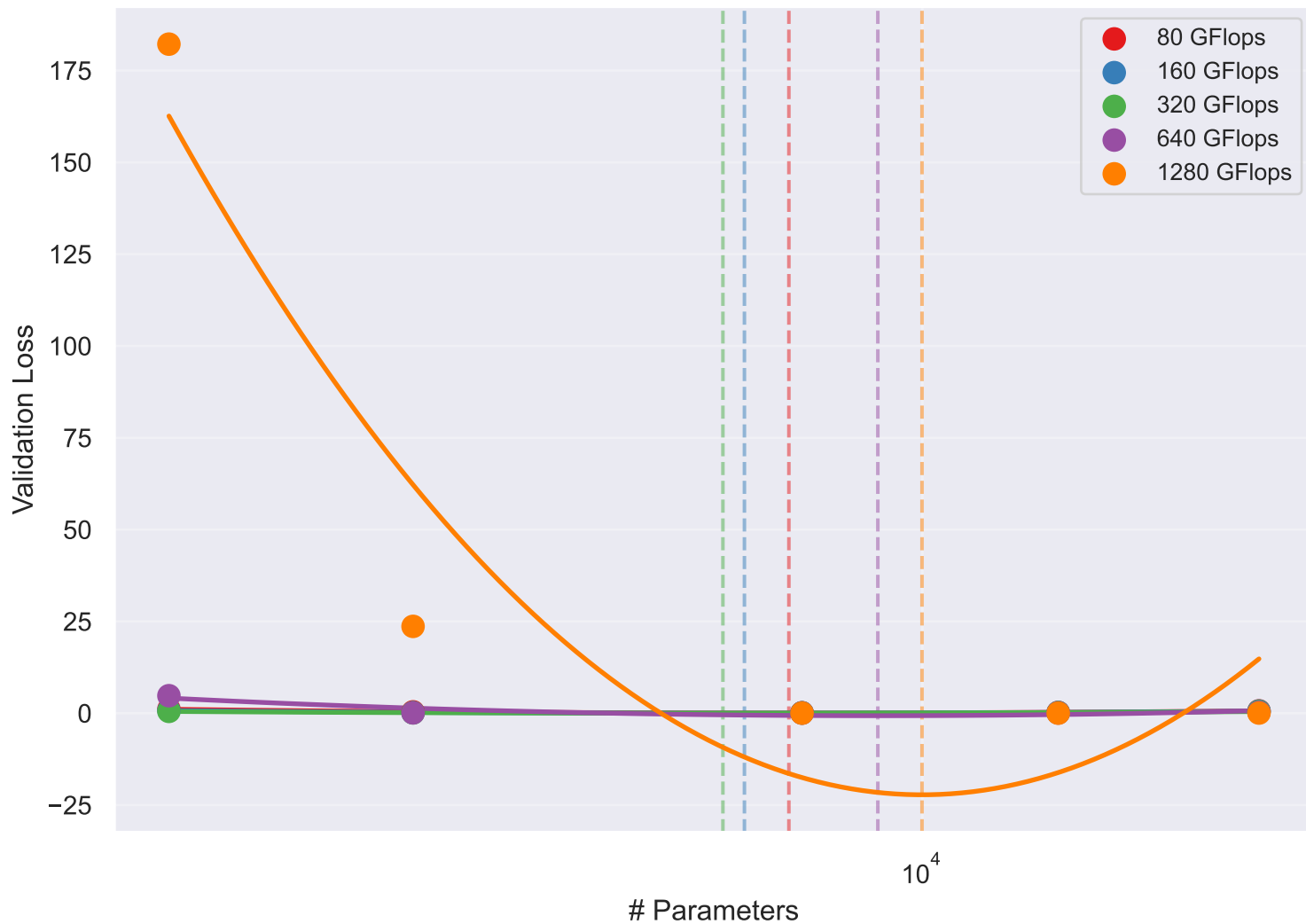
IsoFLOP Analysis: Optimal Model Size vs Compute Budget
