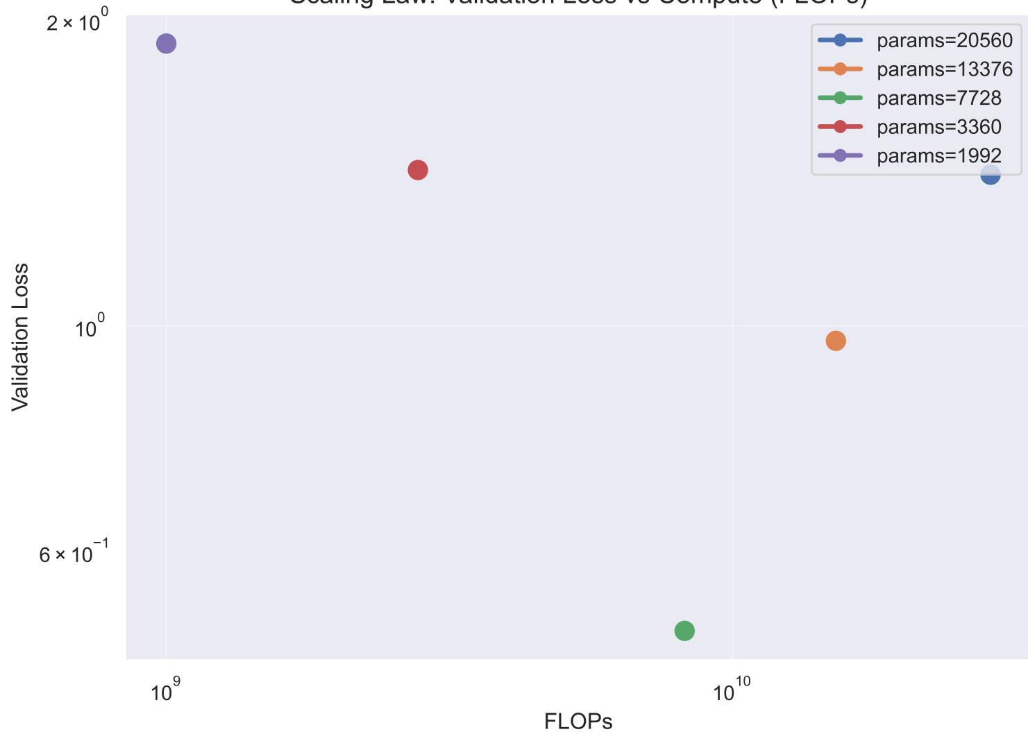
Scaling Law: Validation Loss vs Compute (FLOPs)
