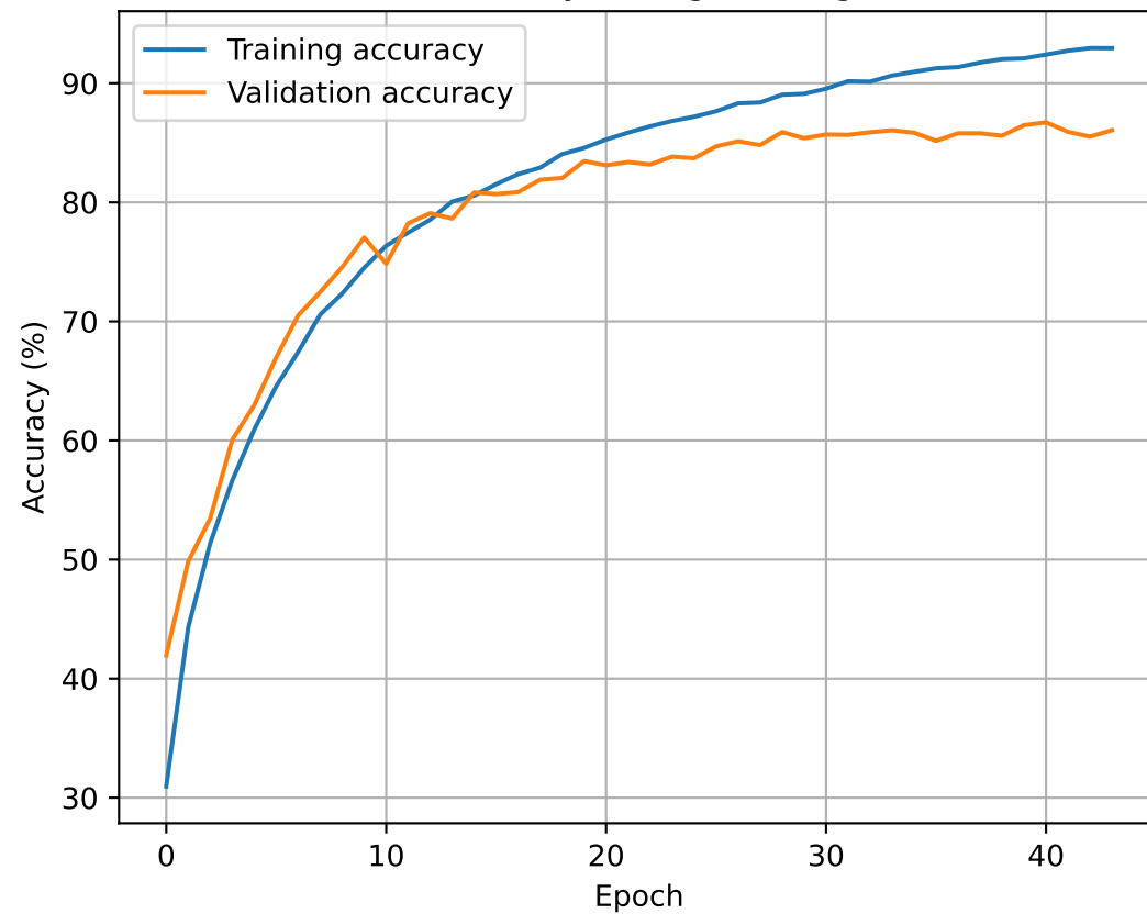
Accuracy during training
