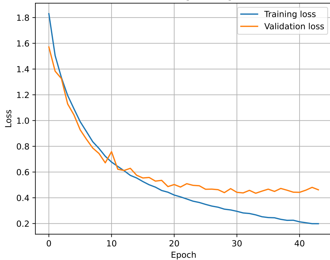
Loss during training
