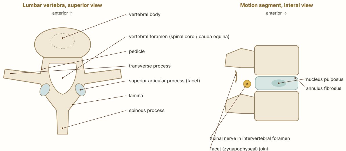
Figure 17.2 A lumbar vertebra from above and a spinal motion segment from the side (schematic). Each segment moves at three joints: the intervertebral disc in front and the paired facet joints behind (Bogduk, 2005).
