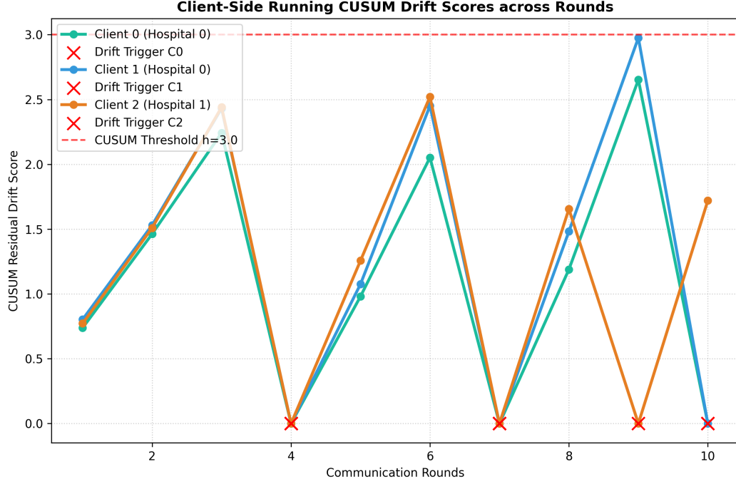
Figure 2: Client running AD-CUSUM concept drift scores across communication rounds highlighting threshold triggers ( H = 3.0 ).
