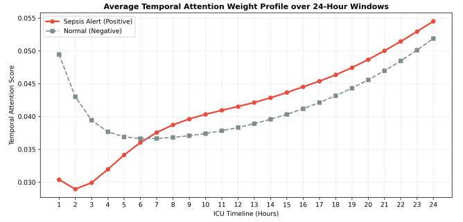
(b) Average Temporal Attention Curve
