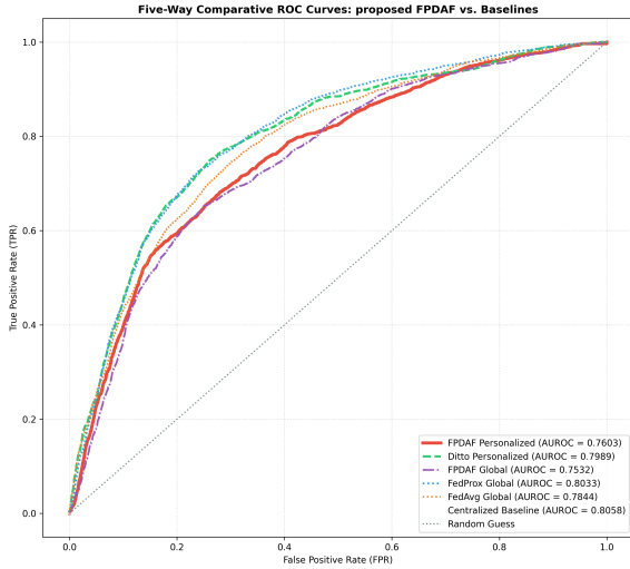
(a) Five-Way ROC Overlay
