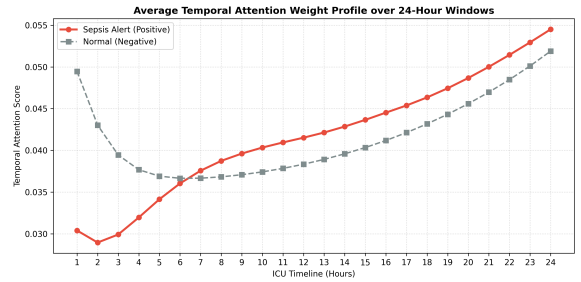
(b) Temporal Attention Profile
