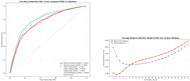
(a) Five-Way ROC Overlay (b) Temporal Attention Curve
