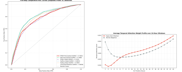
(a) Five-Way ROC Overlay (b) Temporal Attention Curve Fig. 11. Clinical explainability and performance overlays.
