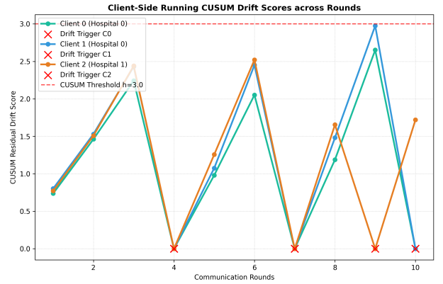
Fig. 10. Client running AD-CUSUM drift scores and trigger points.
