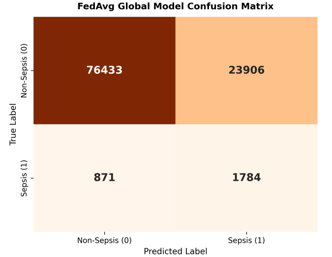
Fig. 4. (Left) Comparative test set ROC curve overlay for FedAvg vs Centralized baseline. (Right) FedAvg global model test confusion matrix heatmap.
