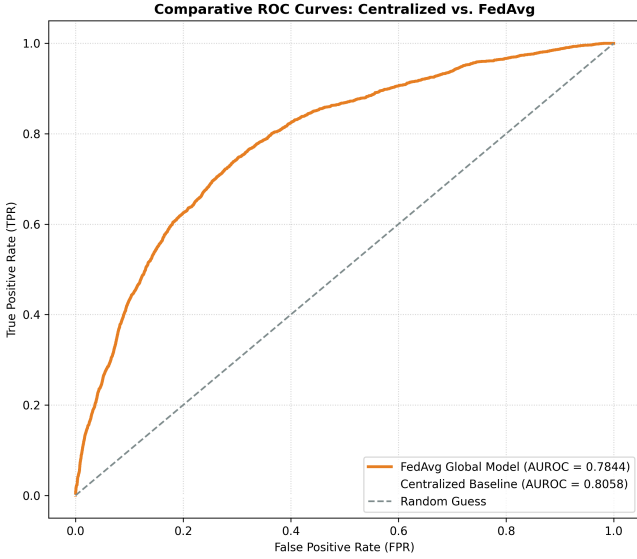
Fig. 4. (Left) Comparative test set ROC curve overlay for FedAvg vs Centralized baseline. (Right) FedAvg global model test confusion matrix heatmap.
