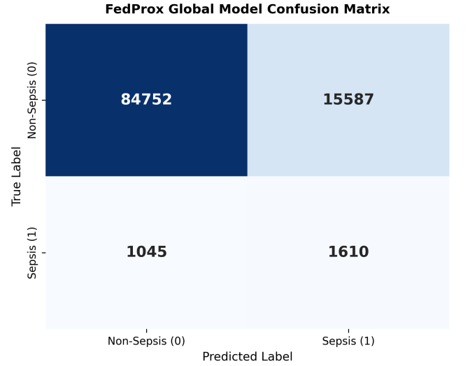
Fig. 6. (Left) Three-way comparative test set ROC curve overlay. (Right) FedProx test set confusion matrix heatmap.
