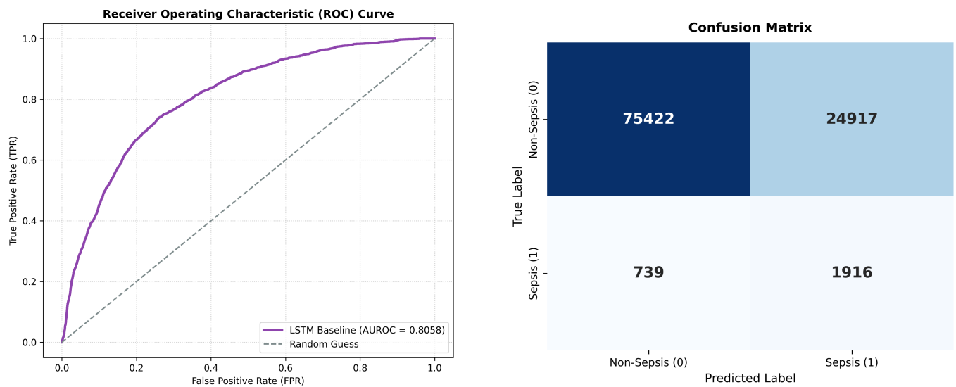
Fig. 2. (Left) Receiver Operating Characteristic (ROC) curve of the baseline model on the test dataset. (Right) Centralized baseline test set confusion matrix heatmap.
