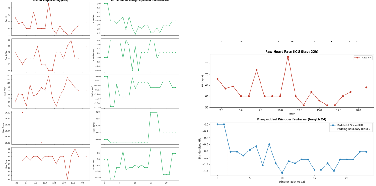
Figure 1: (Left) Vital sign time-series before and after patient-level imputation and leakage-free z-score normalization. (Right) Zero pre-padding validation on a short-stay ICU patient window ( T < 24h ) to form uniform 24-hour sequence matrices.
