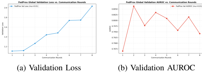
Fig. 7. FedProx global model performance across communication rounds.
