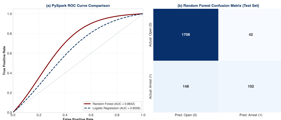
Figure 6: PySpark Machine Learning Model Evaluation: Confusion Matrix and ROC Curve (AUC = 0.8842).
