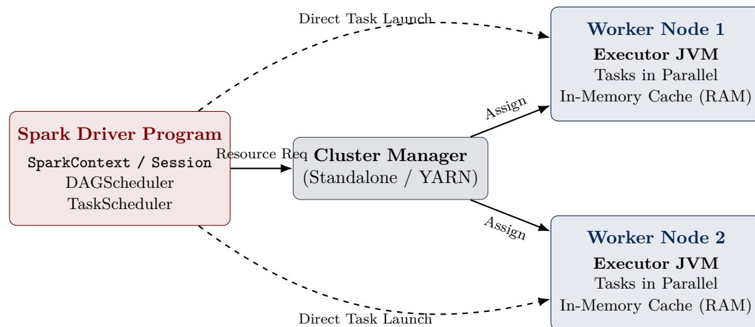
Figure 2: Apache Spark Master-Worker Distributed Execution Architecture.
