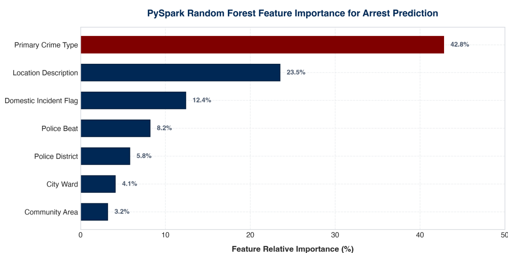
Figure 7: Random Forest Feature Importance Weights for Crime Arrest Predictability.
