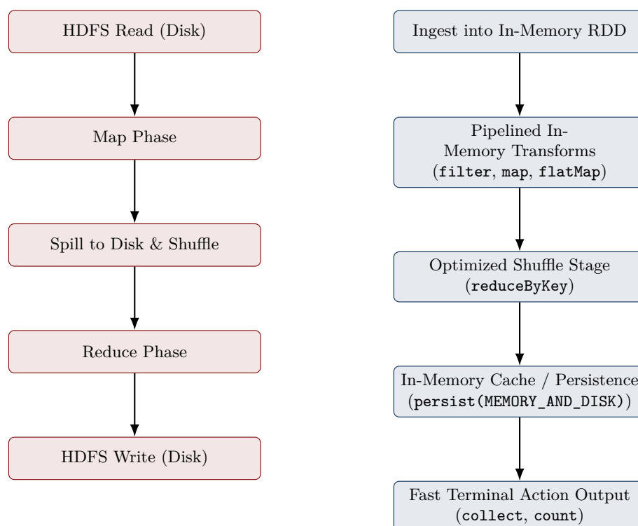
Figure 1: Architectural Comparison: Hadoop MapReduce Disk I/O vs. Apache Spark In-Memory Execution.
