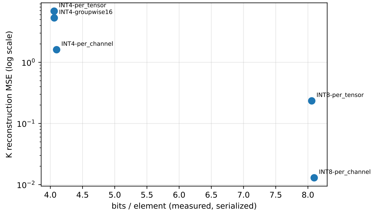
Rate-distortion, K cache (Qwen2.5-0.5B, measured)
