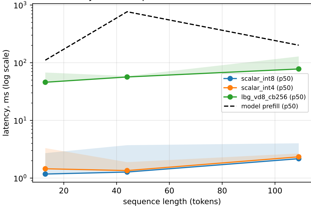
Encode latency vs model prefill - the codec is not the bottleneck
