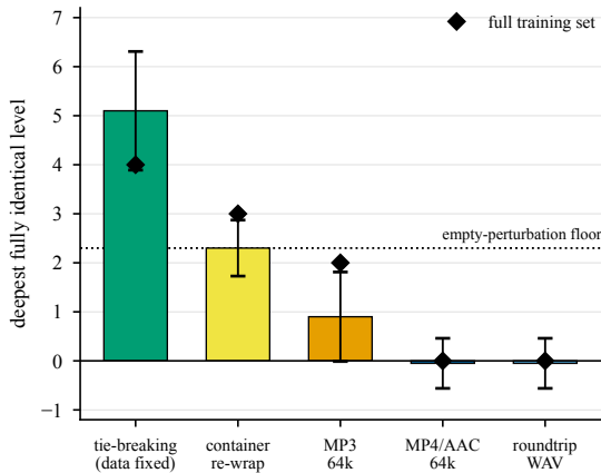
(b) the codecs sit below a floor that carries no information (bars: 20 paired actor draws, mean \pm sd)
