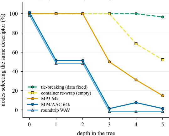
(a) agreement decays with depth, in codec order
