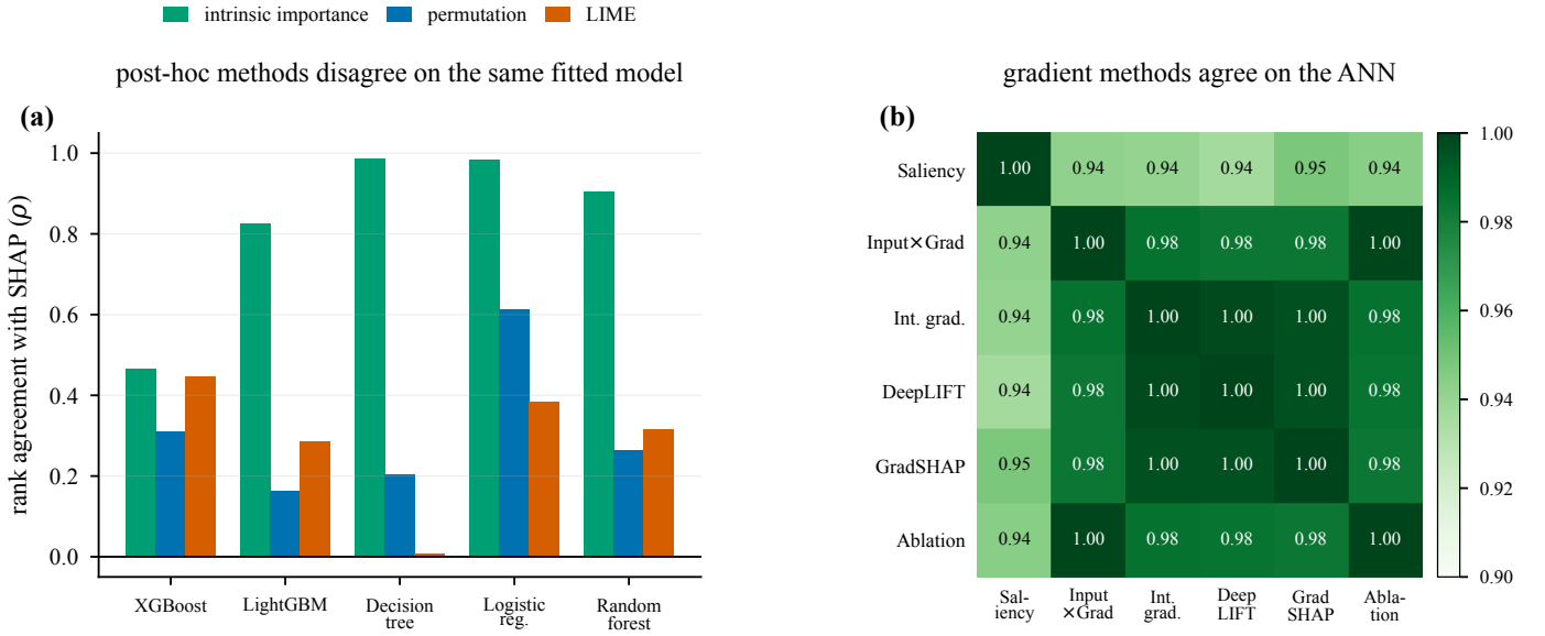
Fig. 8. Agreement between explanation methods, measured as Spearman rank correlation over all 436 descriptors. (a) Post-hoc methods applied to the same fitted tabular model. SHAP tracks intrinsic importance closely for the simpler models, while LIME and permutation importance are nearly unrelated to it. On the decision tree, LIME and SHAP agree at only \rho = 0.008 . (b) The six methods of the gradient family, applied to the network, agree almost perfectly, at \rho \geq 0.94 for every pair. This shows that the disagreement in panel (a) is a property of the method families rather than of this feature space.
