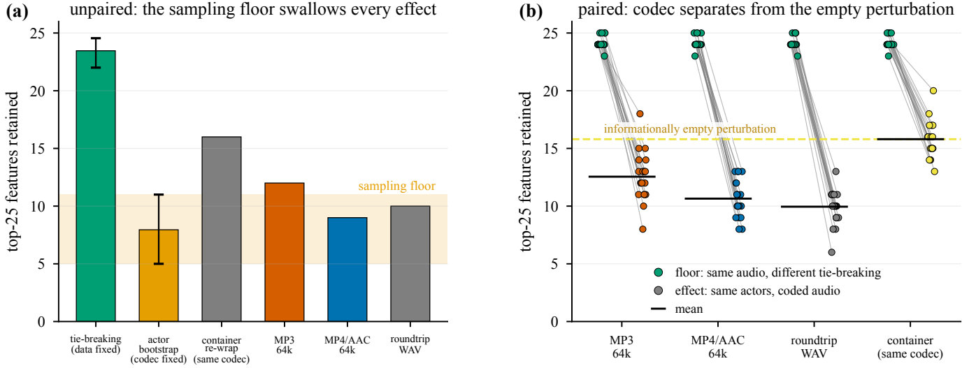
Fig. 7. A codec effect on a feature-importance ranking cannot be interpreted without a null. (a) When the comparison is made marginally, the actor-resampling floor is so wide that every codec effect falls inside it. (b) When floor and effect are measured inside the same resampled training set, using 20 draws of 51 of the 60 training actors and computing both quantities on the same draw, the codec effect separates cleanly. The decisive control is the rightmost group. An informationally empty container re-wrap already costs 8.4 of the 25 descriptors, so only the gap between that line and the codec bars can be attributed to the codec.
