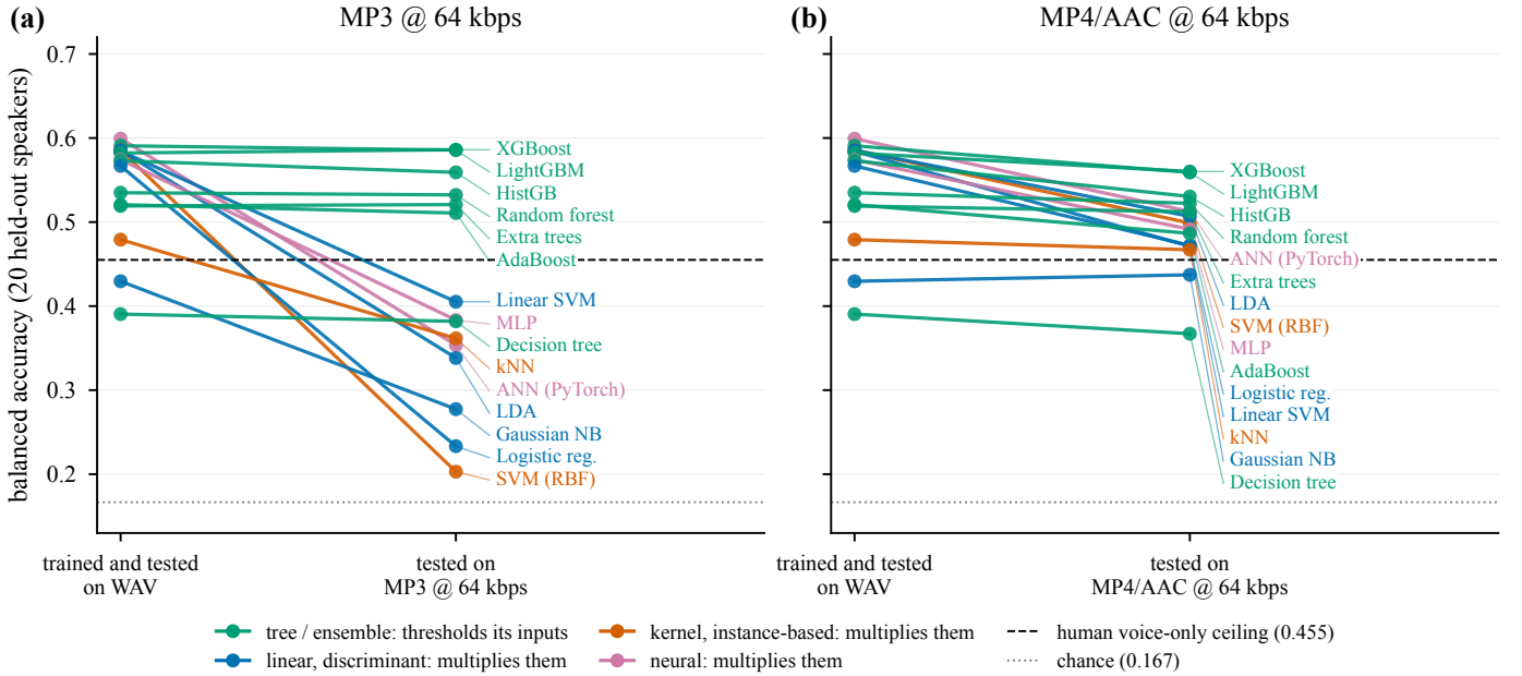
Fig. 3. Robustness to lossy coding under train/serve mismatch is determined by how a model consumes its inputs, and not by how accurate that model is. (a) Under MP3 at 64 kbit s -1 the tree family stays flat, while the magnitude-sensitive family falls through the human ceiling and towards chance. (b) Under MP4/AAC the same models degrade broadly and mildly, which is consistent with a diffuse frame-alignment perturbation rather than with the failure of a single band. All models were trained on uncompressed audio only.
