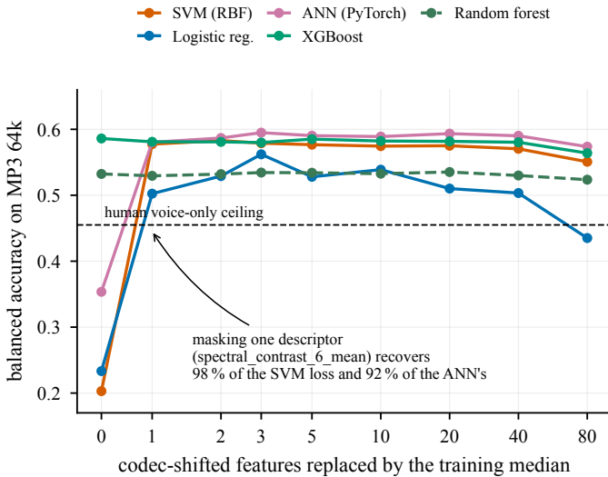
Fig. 10. Neutralisation on MP3 at 64\text{ kbits}^{-1} , which replaces the most codec-shifted descriptors with their training medians. Masking a single descriptor recovers almost the entire collapse for every affected model. The tree models were never affected and stay flat throughout. Beyond roughly 20 descriptors the masking begins to destroy real evidence. On uncompressed audio the same masking costs nothing out to 20 descriptors, which confirms that these columns never carried load-bearing evidence.
