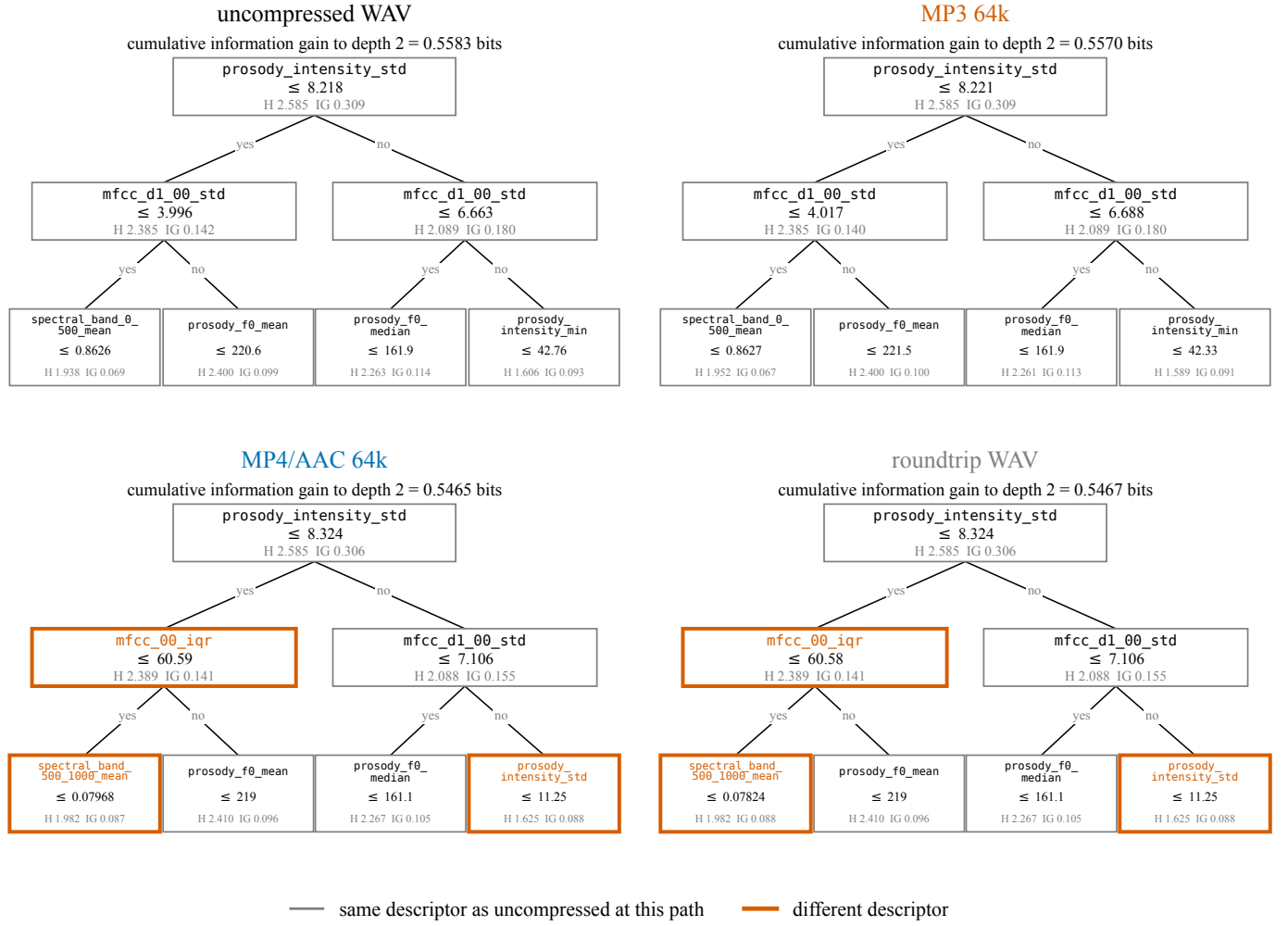
Fig. 5. The top three levels of the entropy tree, fitted separately on each condition using the same actors and the same items. Every node carries its own entropy H and its information gain, both in bits, so the calculation of Eq. 2 and Eq. 3 is shown at each node rather than only at the root. The identity of the root test does not change with the codec, and its threshold and information gain change very little. The trees begin to diverge one level below the root, and they diverge under AAC rather than under MP3. The AAC and roundtrip trees abandon the frame-aligned delta descriptor \text{mfcc\_d1\_00\_std} in favour of the static dispersion measure \text{mfcc\_00\_iqr} , which is what the 32.68ms priming shift predicts. AAC and roundtrip carry the same codec output through two different containers, and they select identical descriptors at all seven nodes shown. The four trees also harvest almost the same cumulative information gain over these three levels while testing different descriptors, which is the result Section VI-F carries down to depth 6.
