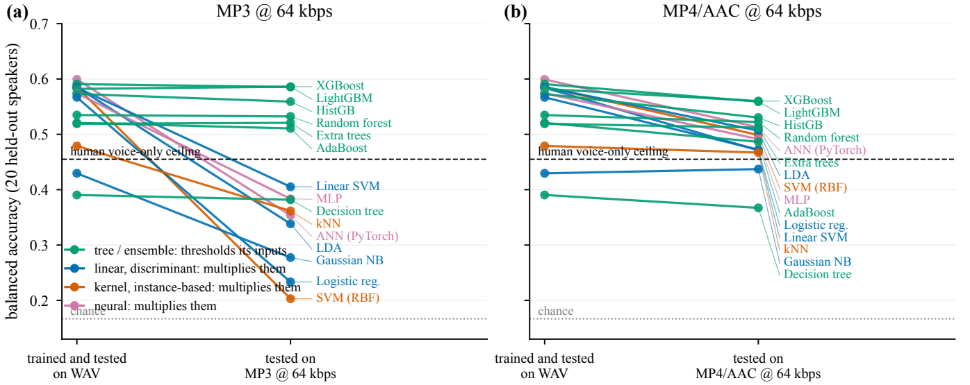
Fig. 3. Robustness to lossy coding under train/serve mismatch is determined by how a model consumes its inputs, and not by how accurate that model is. (a) Under MP3 at 64 \text{ kbit s}^{-1} the tree family stays flat, while the magnitude-sensitive family falls through the human ceiling and towards chance. (b) Under MP4/AAC the same models degrade broadly and mildly, which is consistent with a diffuse frame-alignment perturbation rather than with the failure of a single band. All models were trained on uncompressed audio only.
